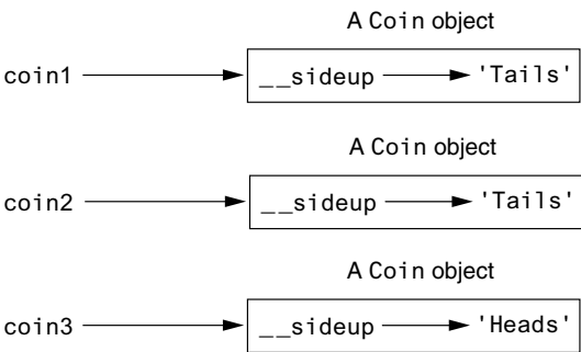
Figure 10-9 The objects after the toss method
