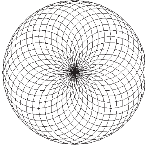
Program 4-22 (spiral_circles.py)
