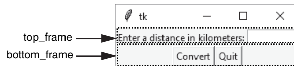
Figure 13-14 The window organized with frames
